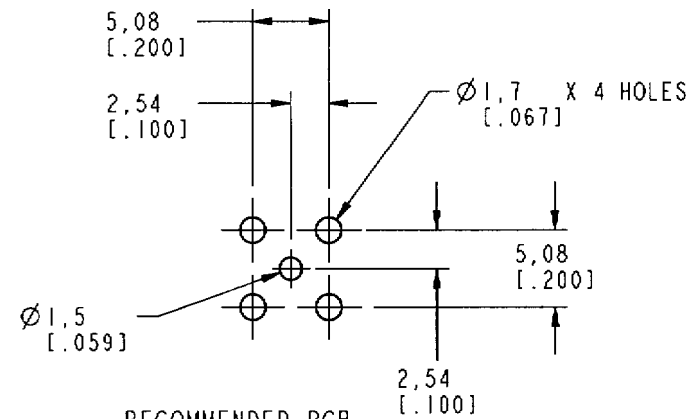
RECOMMENDED PCB MOUNTING HOLE SCALE 2.000
